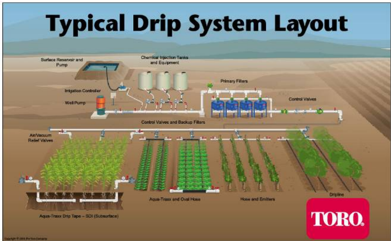
Figure 1: Typical Drip System Layout
